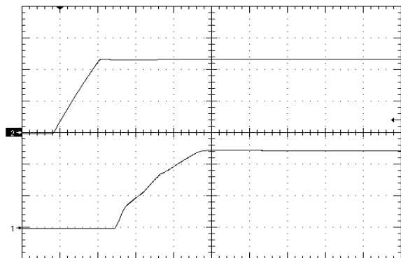
Figure 10. Startup Waveform via Line Voltage, time scale 4mS/div. Vin=Vin_nom, Iout=full load Cout=0µF, Ch1=Vout (2V/div), Ch2=Vin (20V/div)
