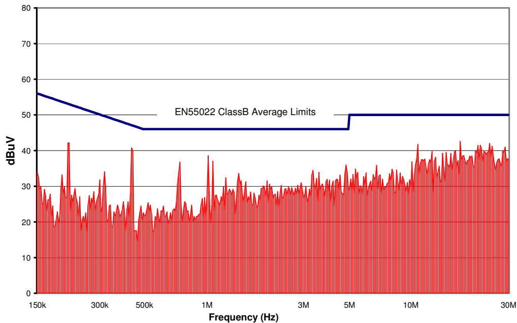
Figure 20. CP15_1130036 Conducted Emissions using above specified input filter. Vin = 48V, Full Resistive Load
