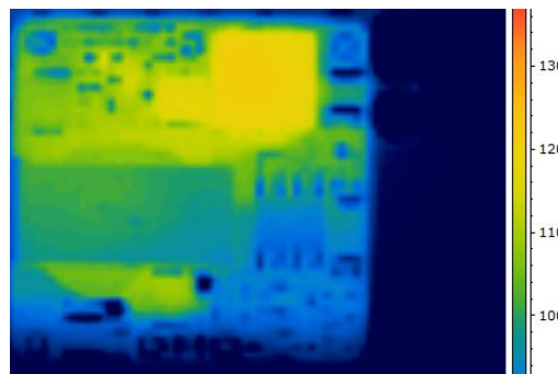
Figure 6. Thermal Image of CP15B1130036 3A output, 85C Ambient, 200lfm airflow, Vin = 48V, T max = 121 °C
