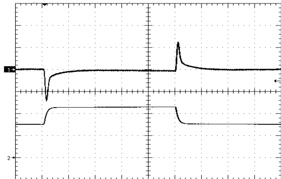
Figure 12. Load Transient Response (50mV/div), di/dt=0.1A/µS, 50%-75%-50% of full load, Cout=Fig16 time scale: 200µS/div. Ch1=Vout, Ch2=Iout (1A/div)
