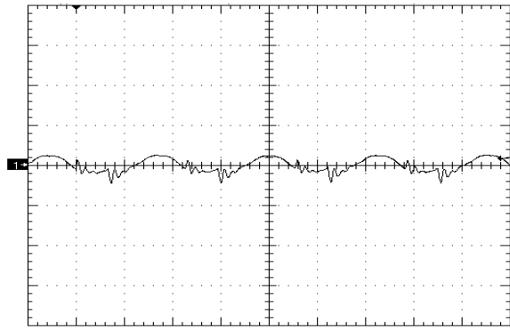
Figure 8. . Output Voltage Ripple (20mV/div), time scale – 1µS/div. Vin=Vin_nom, full load Cout=1µF ceramic + 10µF Tantalum (see Fig 16)
