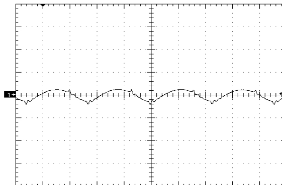
Figure 8. Output Voltage Ripple (50mV/div), time scale – 1uS/div. Vin=Vin_nom, full load Cout=1uF ceramic + 10uF Tantalum (see Fig 16)
