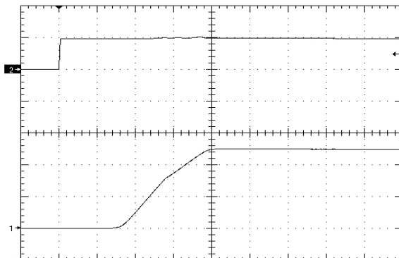
Figure 11. Startup Waveform via Enable Pin, time scale 4mS/div. Vin=Vin_nom, Iout=full load Cout=1000uF, Ch1=Vout (2V/div), Ch2=enable (5V/div)
