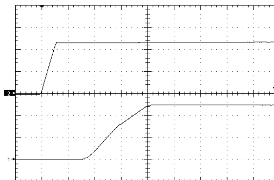
Figure 10. Startup Waveform via Input Voltage, time scale 4mS/div. Vin=Vin_nom, Iout=full load Cout=1000uF, Ch1=Vout (2V/div), Ch2=Vin (10V/div)
