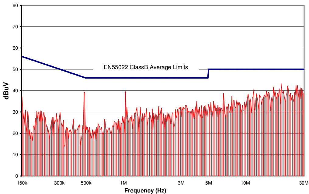
Figure 20. CP15_1130018 Conducted Emissions using above specified input filter. Vin = 24V, Full Resistive Load
