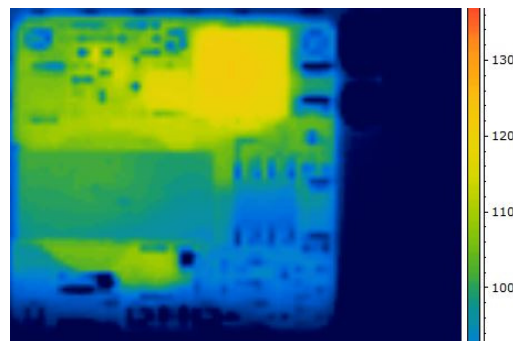
Figure 6. Thermal Image of CP15B1130018 3A output, 85C Ambient, 200lfm airflow, Vin = 24V, T max = 121 °C
