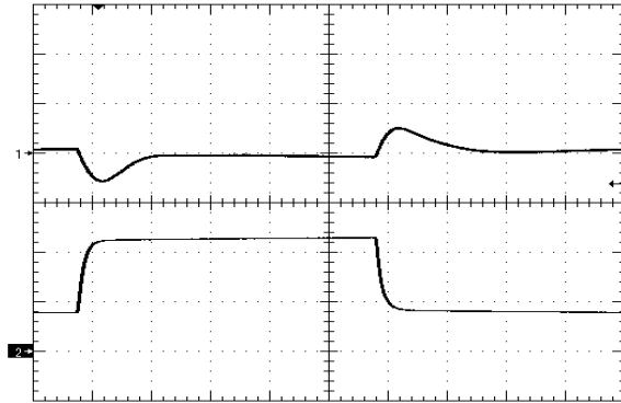
Figure 14. Load Transient Response 50mV/div), di/dt=0.2A/uS, 25% - 75% - 25% of full load +1000uF low ESR Oscon, time scale: 200uS/div. Ch1=Vout, Ch2=Iout (1A/div)
