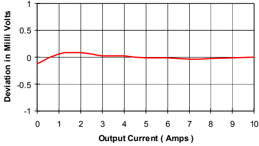
Load Regulation
