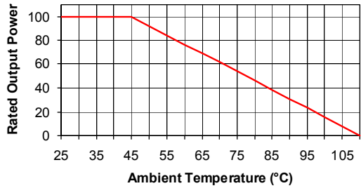
Output Load Vs Ambient. Natural Convection
