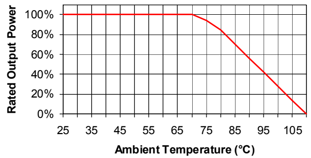
Output Load Vs Ambient. Natural convection
