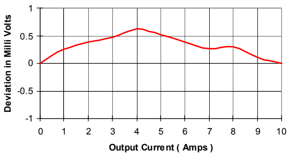
Load Regulation
